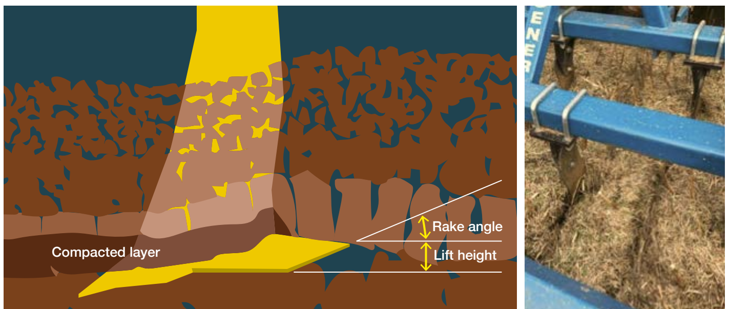
Figure 14. Geometry of loosening parts and minimal surface disturbance (left). Sufficient lift to create vertical fissures is needed at the problem depth. Low rake angles minimise surface disruption and heave, provided lift height is adequate for fissure creation. Sideways inclined legs (right) can also minimise surface disturbance, provided operational speeds are appropriate
